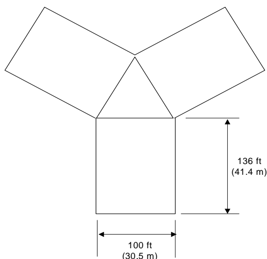
Figure 4-5. Gravity anchor
