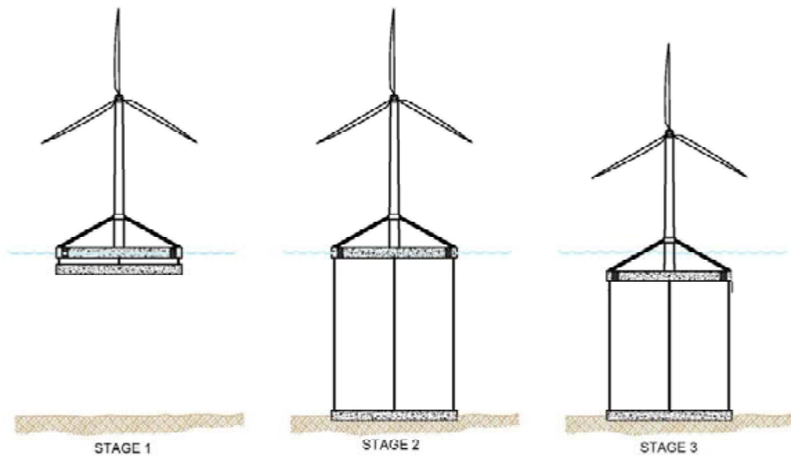
Figure 4-7. Installation sequence
