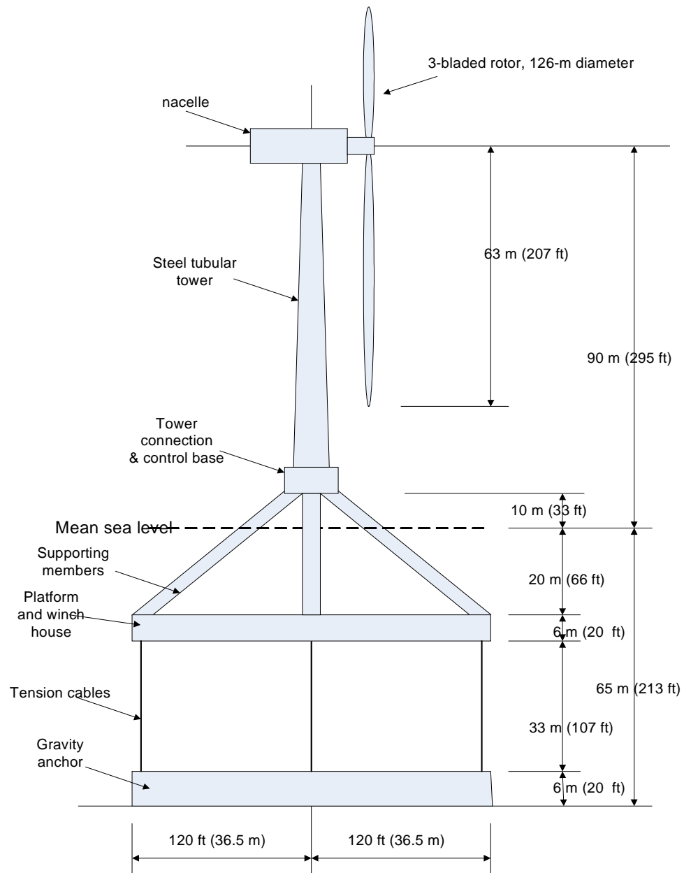
Figure 4-2. Submerged TLP
