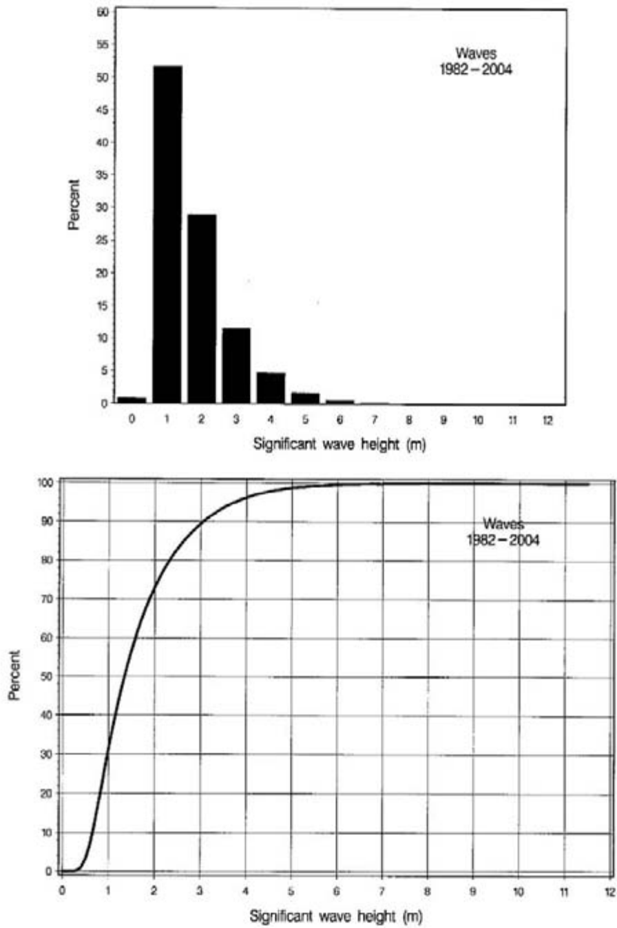
Figure 2.1.3. Histogram of significant wave height, all data (top), and cumulative percentage of significant wave height, all data (bottom).
