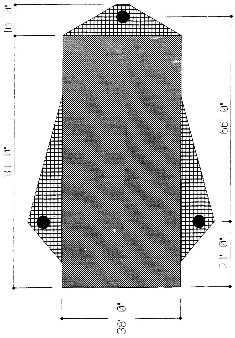
GENERIC LIFTBOAT - PLAN VIEW STEWART TECHNOLOGY ASSOCIATES October 31, 1989 | FIGURE 1
